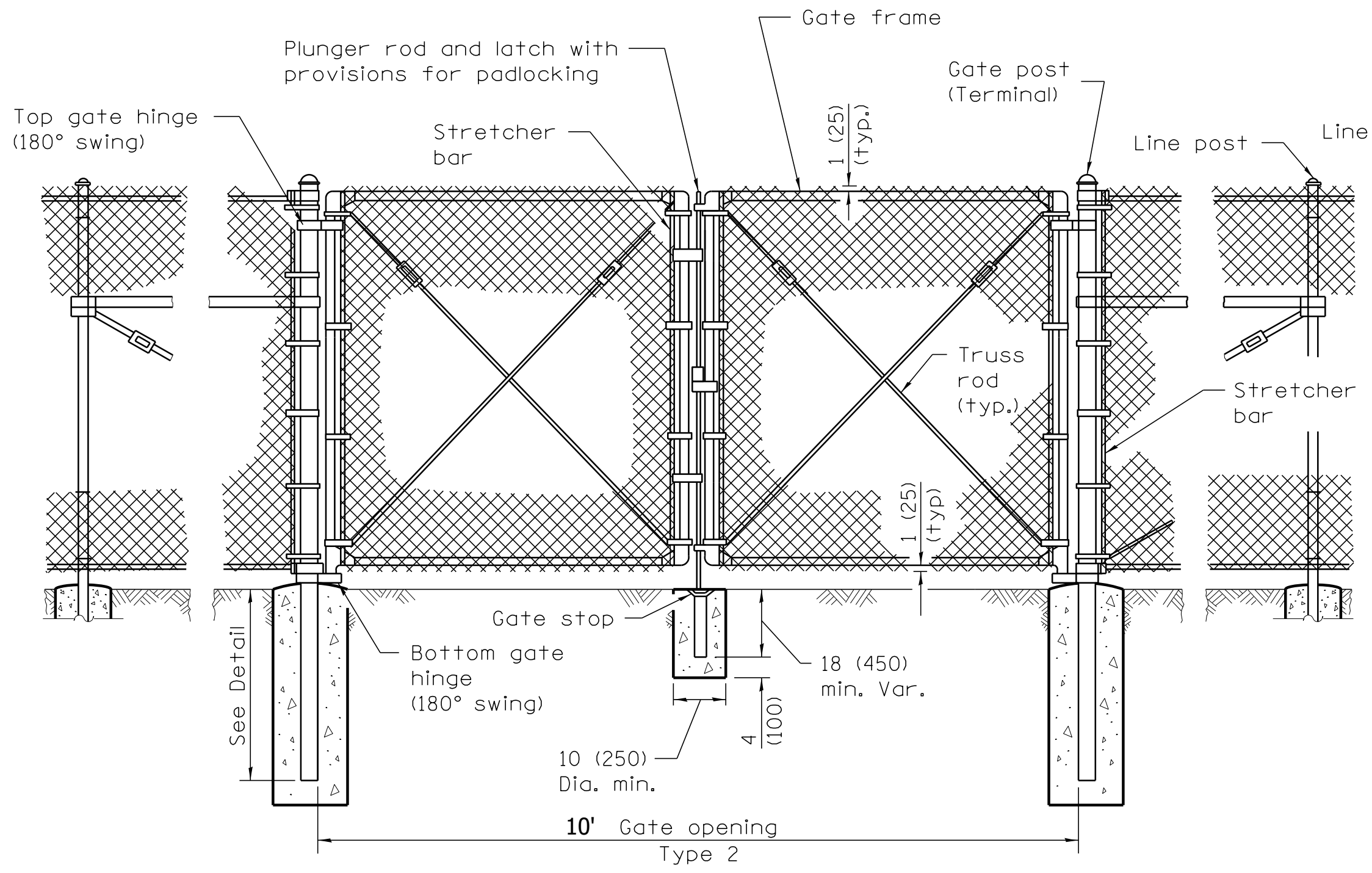
VEHICLE GATE ARRANGEMENT
