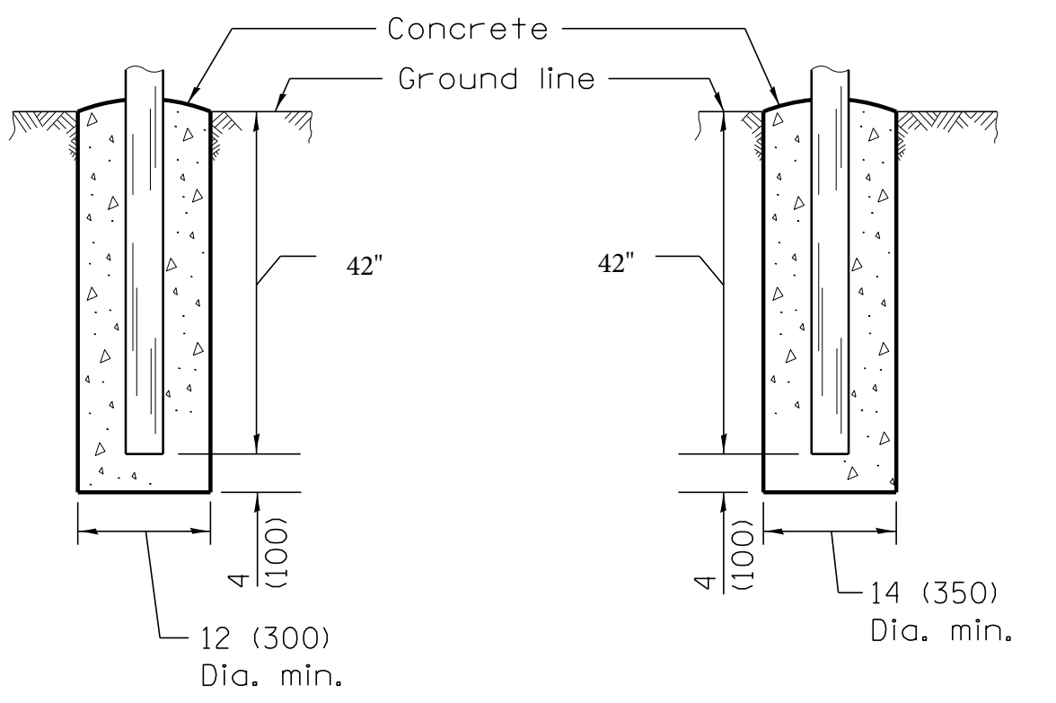
FOOTING FOR LINE POST
