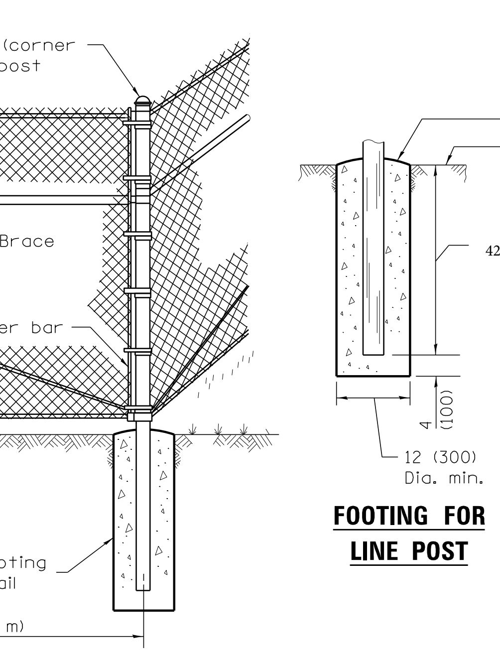
CORNER OR END POST ARRANGEMENT
