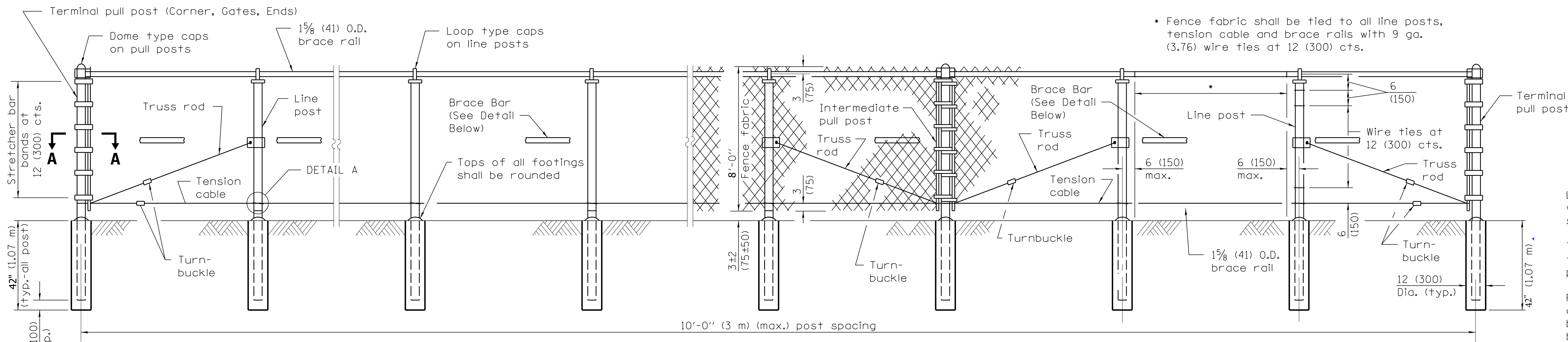
ELEVATION - ( 8' ) FENCE (Looking toward tree-line )
