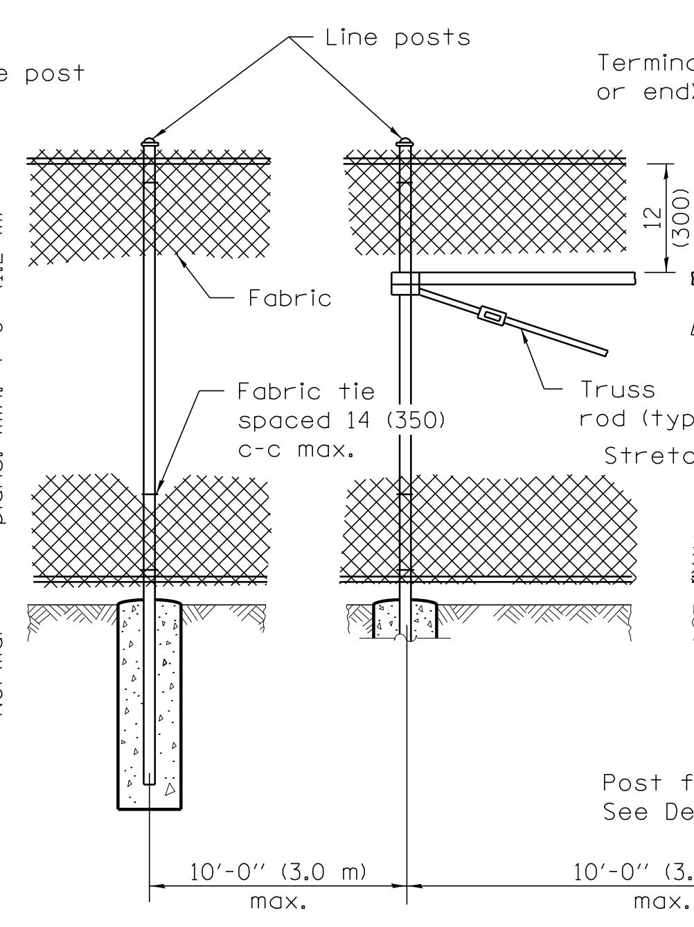
LINE POST ARRANGEMENT
